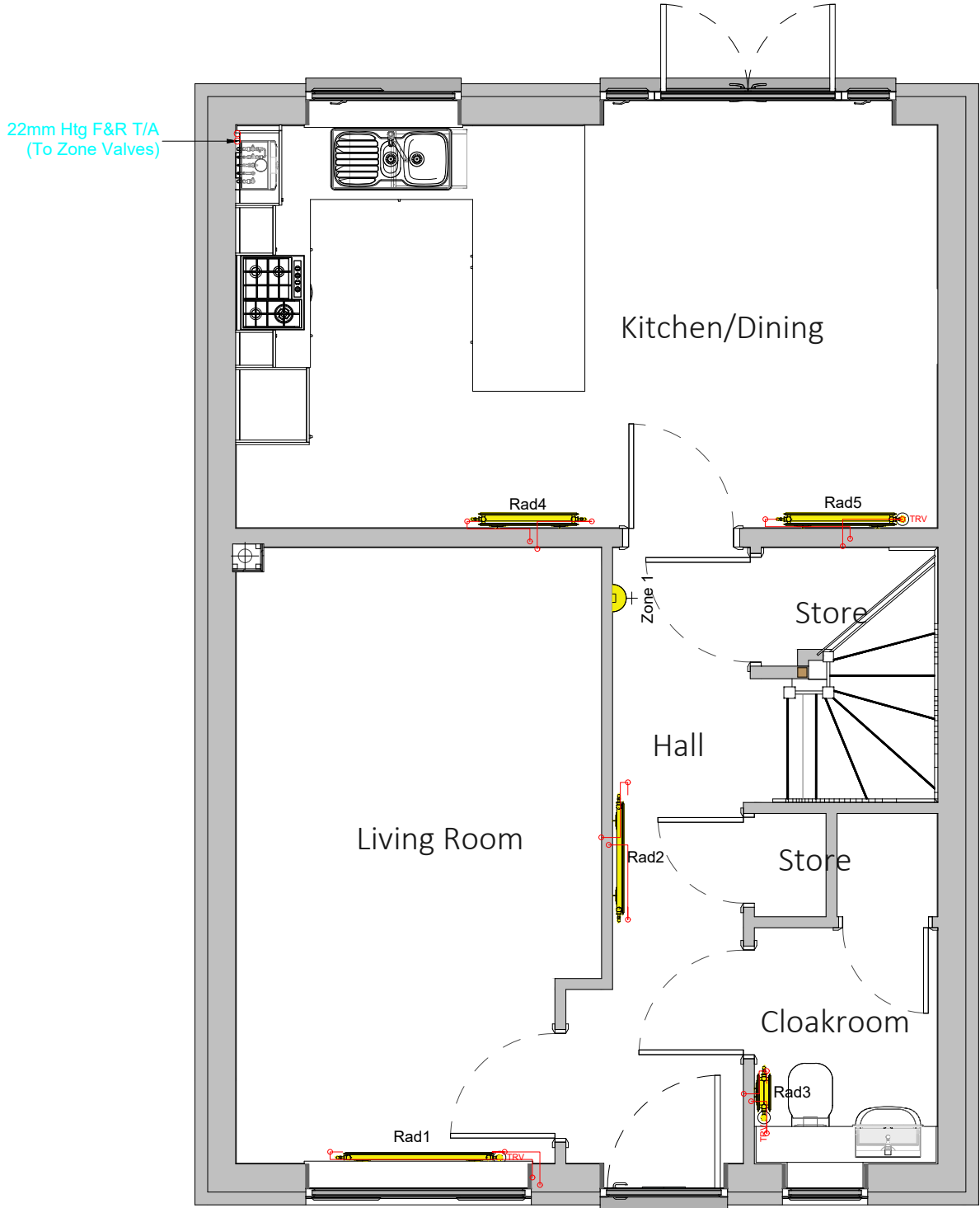
1 Ground Floor Heating GA 1 : 50
